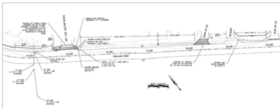
Drainage Improvements, Shoalwater Bay Reservation, Tokeland, Washington; Shoalwater Bay Tribe
